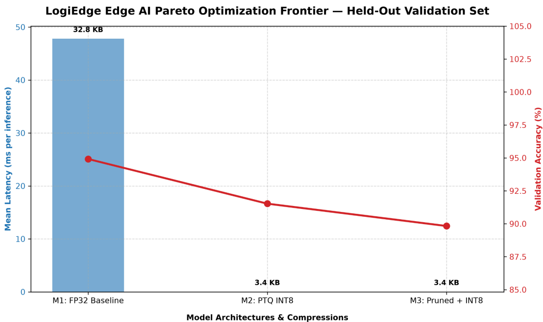
Figure 2: Pareto optimization frontier illustrating the trade-offs between model latency, storage
